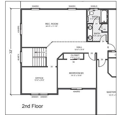
Alternate Rec. Room Layout
