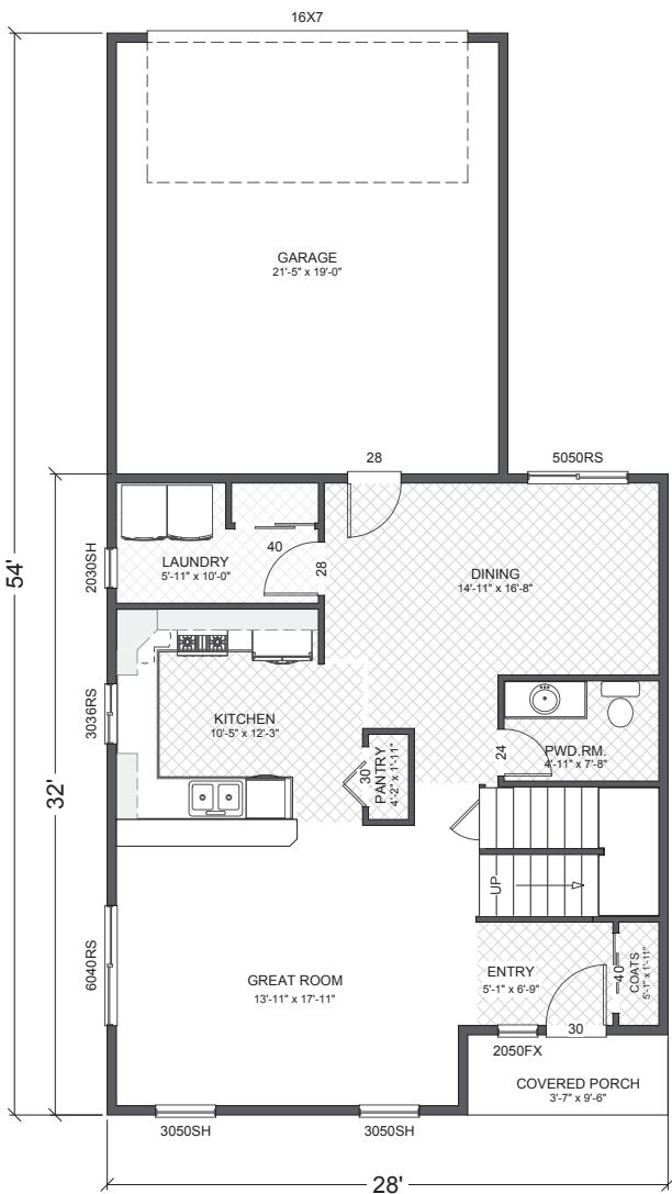
1st Floor
