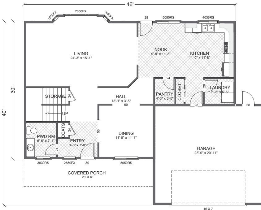
1st Floor
